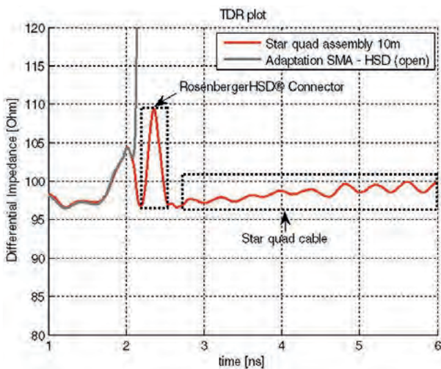
Figure 14: TDR plot of a star quad-cable
